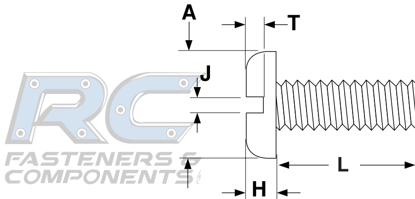
NYLON PAN HEAD MACHINE SCREWS
