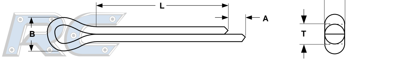
COTTER PINS - EXTENDED PRONG, CHISEL POINT
