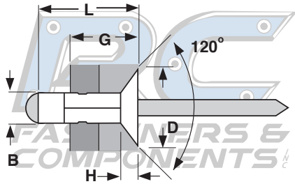
COUNTERSUNK
