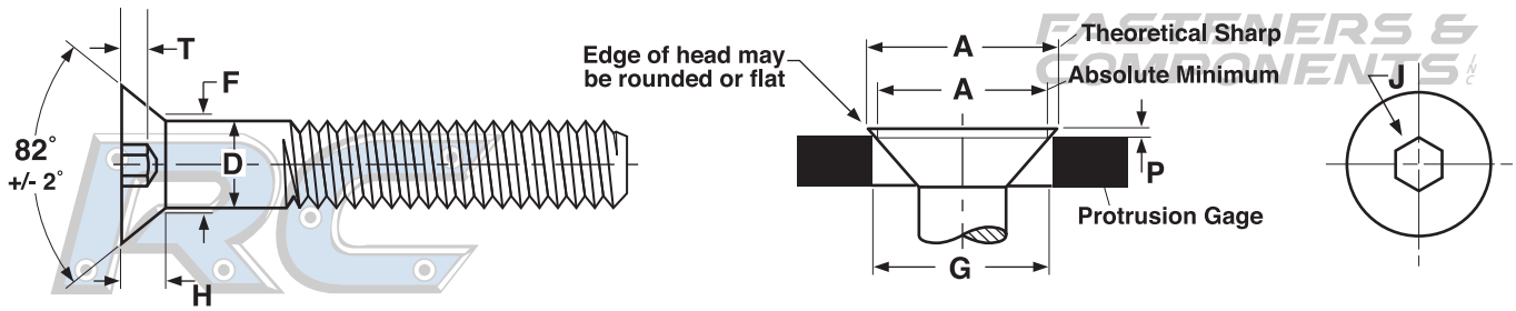
SOCKET FLAT HEAD CAP SCREWS - ALLOY STEEL ASME B18.3-2012, Blue Devil®
