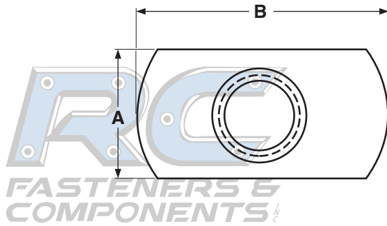
WELD NUTS, CENTER HOLE DESIGN WITHOUT PROJECTIONS
